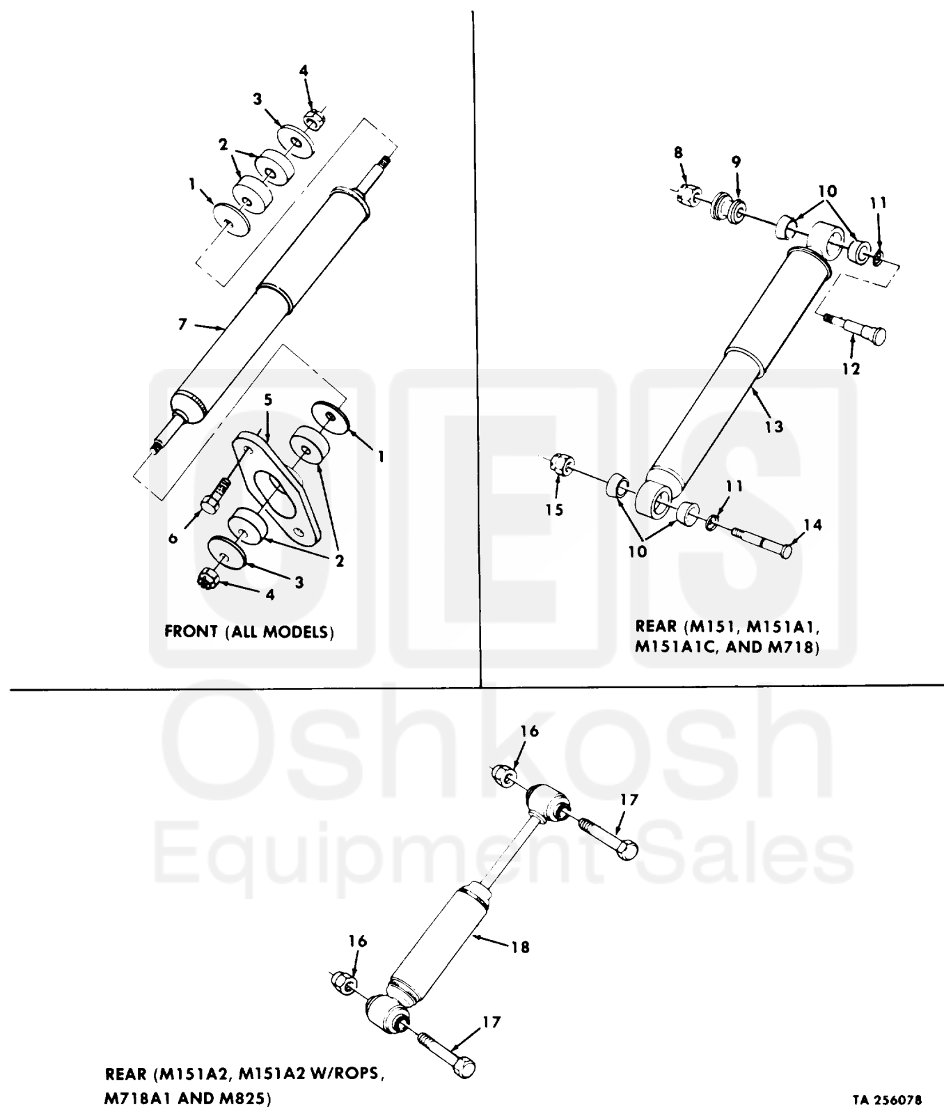
Figure 99. Shock Absorbers and Mounting Parts.
